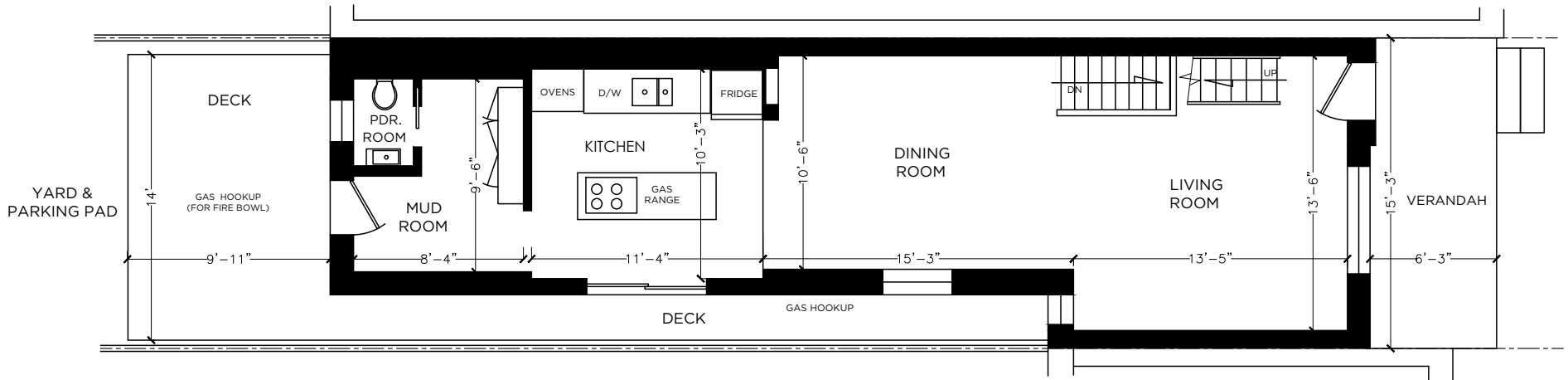
MAIN FLOOR FLOOR AREA 685 SQUARE FEET
