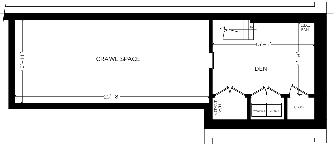
BASEMENT FLOOR AREA 236 SQUARE FEET
