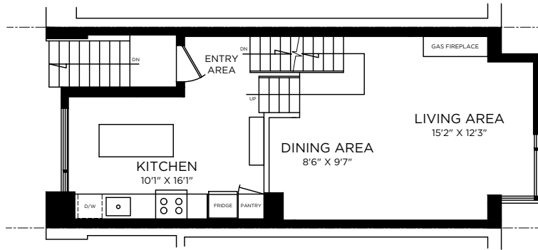
MAIN FLOOR
