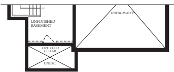
Basement Elevation B
