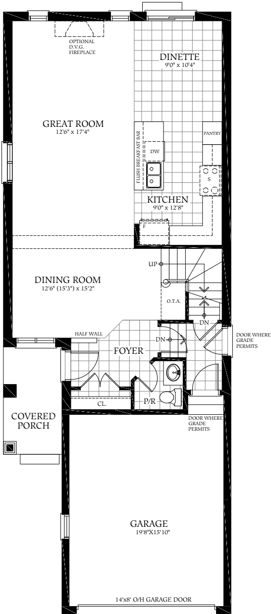
Ground Floor Elevation A
