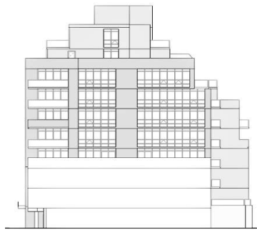
SOUTH ELEVATION
