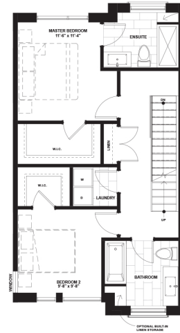
SECOND FLOOR OPTION 2
