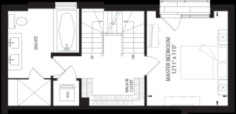
FORTH FLOOR
