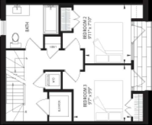
FOURTH FLOOR
