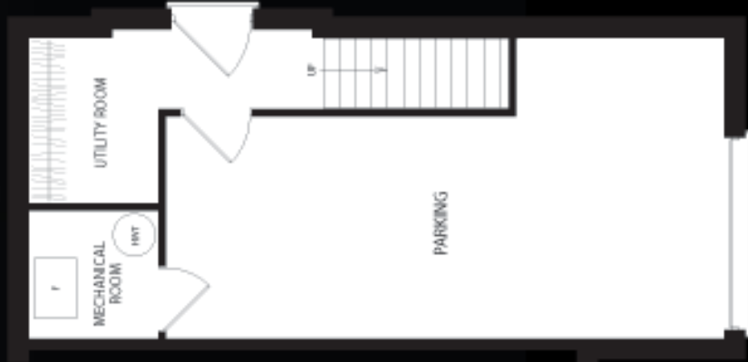
PARKING LEVEL
