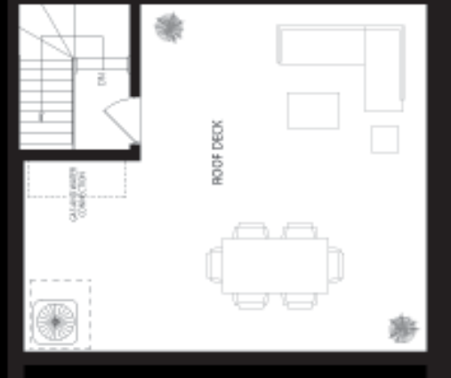
ROOF PLAN
