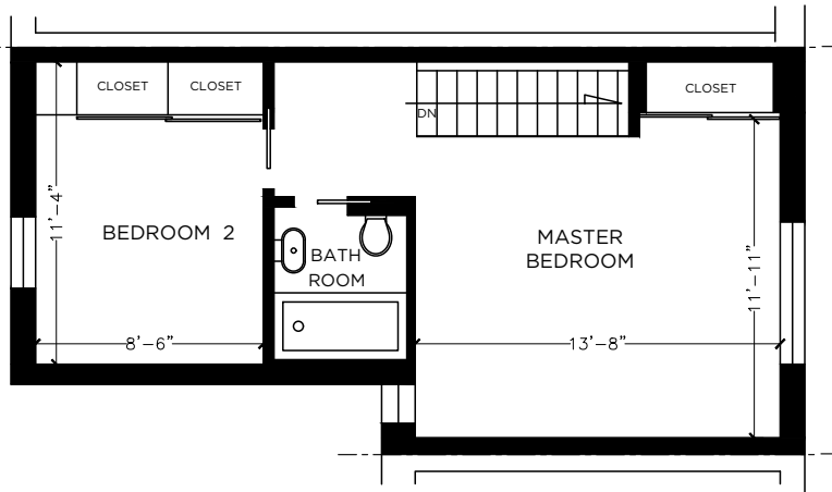
SECOND FLOOR FLOOR AREA 414 SQUARE FEET
