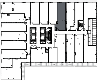
TYPICAL FLOORS 3-7
